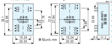
封装尺寸图Size dimensional drawing
