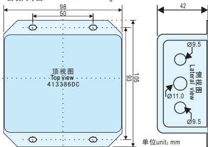
封装尺寸图Size dimensional drawing
