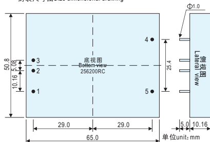
封装尺寸图Size dimensional drawing
