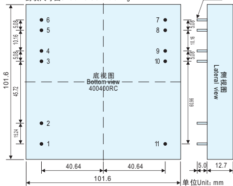
封装尺寸图Size dimensional drawing
