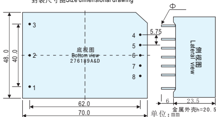
封装尺寸图Size dimensional drawing
